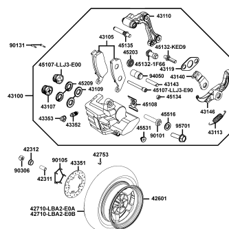
F08 Rear Wheel
